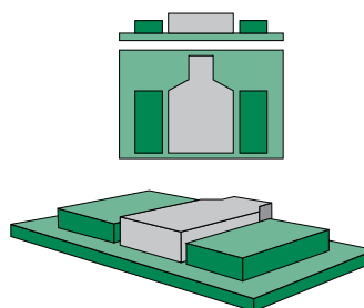
Figure 1.9: NSMD pad
