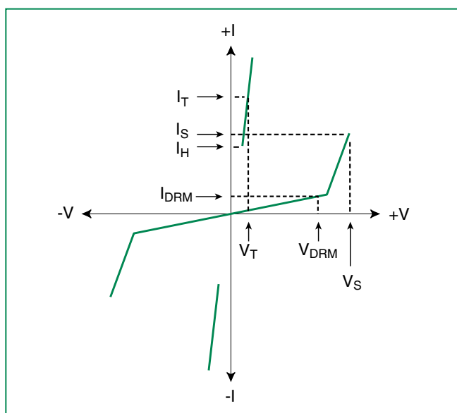
Figure 1.3 V-I Characteristics
